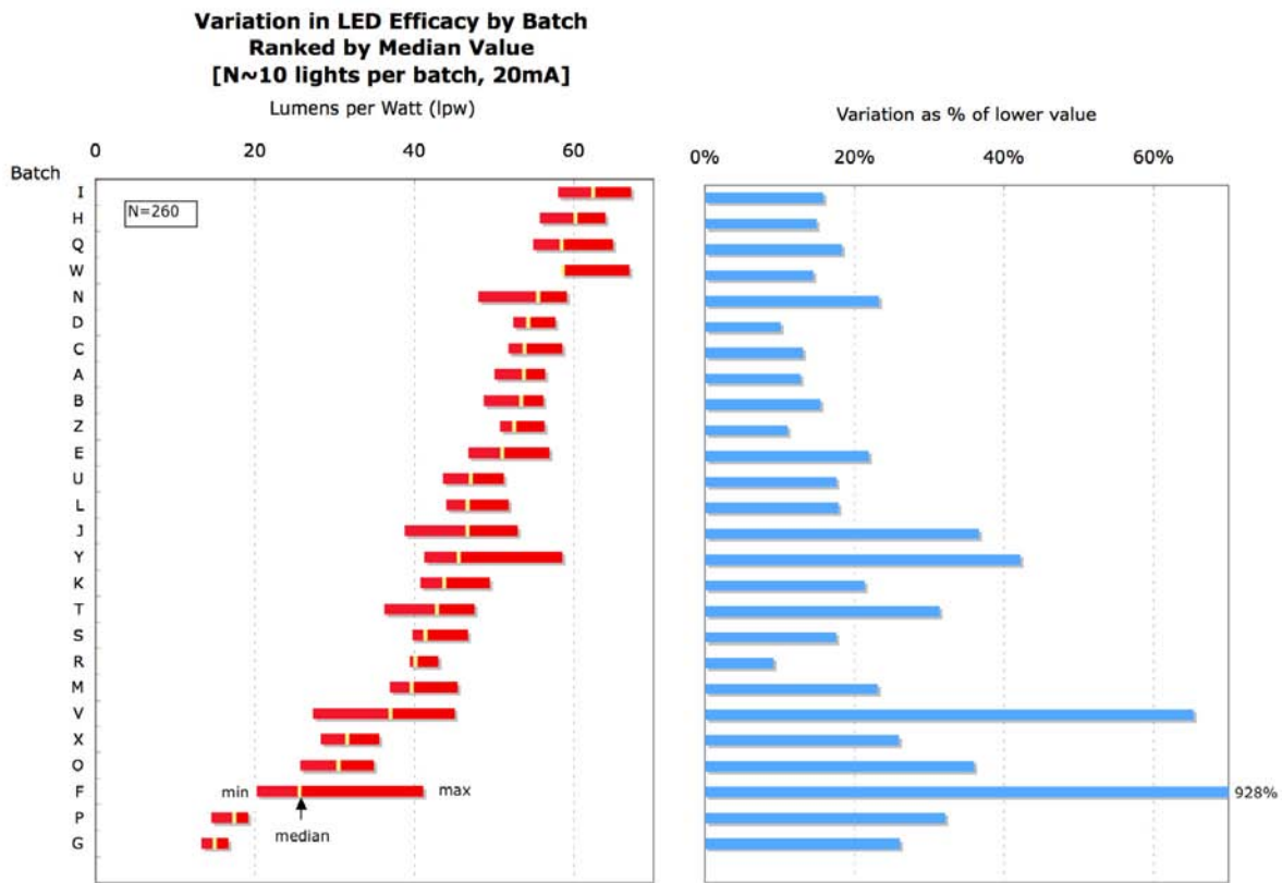
Figure 4. Variation of Luminous Efficacy within 26 Batches of WLEDs.
